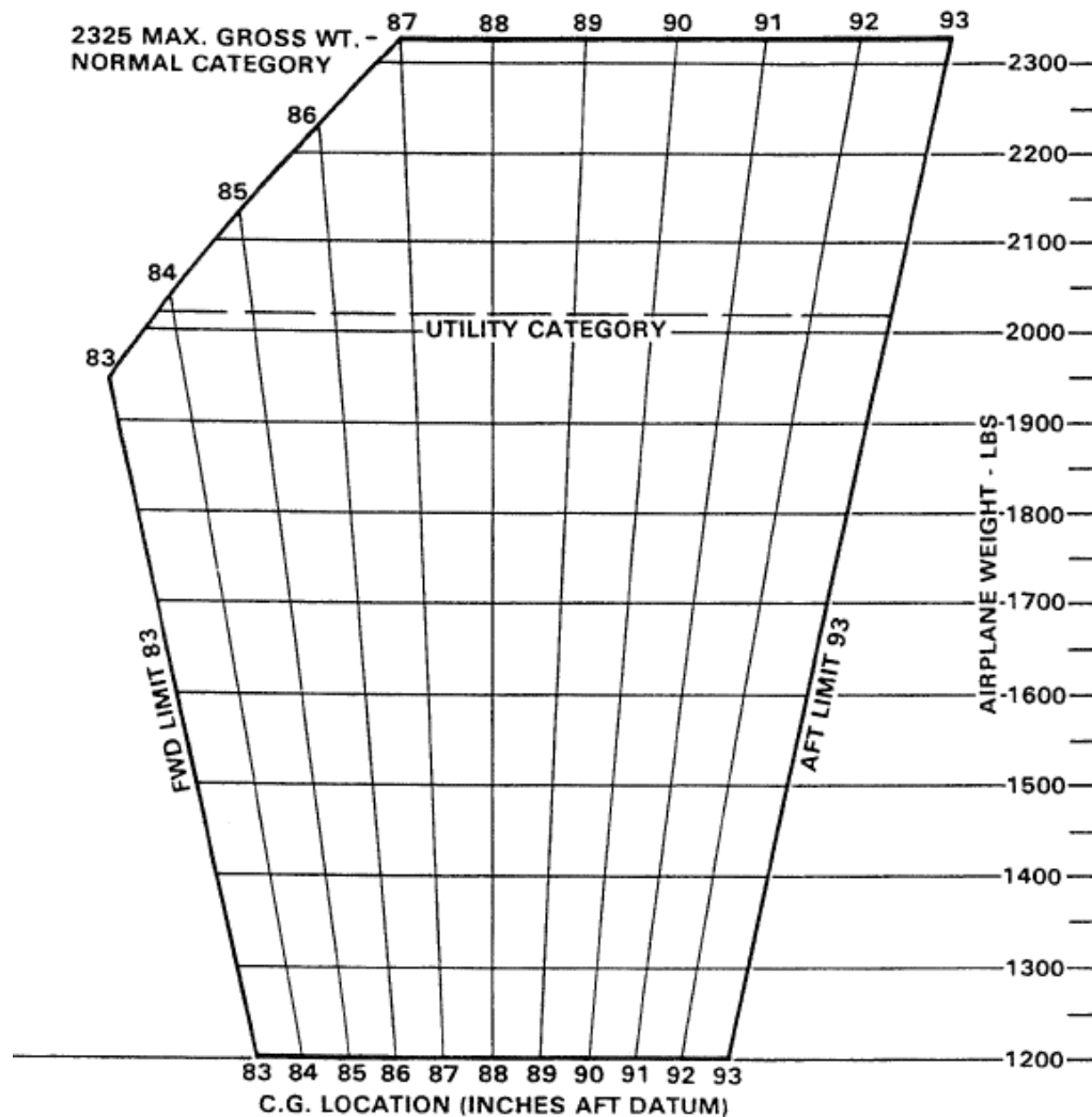
WEIGHT VS C.G. ENVELOPE
